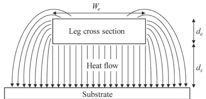
Figure 4: Sidewall thermal conduction model for atmospheric pressure condition.
