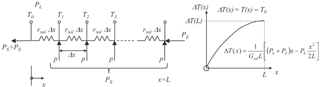
Figure 6: Distributed thermal resistance model for vacuum condition.
