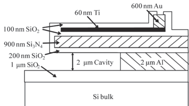
Figure 2: Cross section of bolometer structure.
