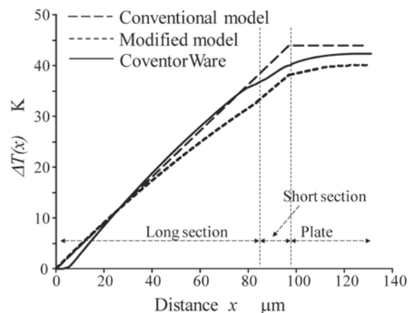
Figure 8: Thermal profiles under vacuum conditions for bolometer device FA1.
