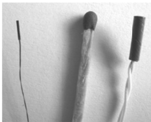
Figure 1: Thin (left) and thick (right) type thermocouples that can be used in grape berry temperature assessment.
