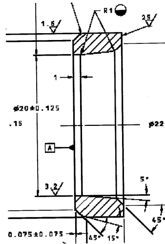
EXHAUST
