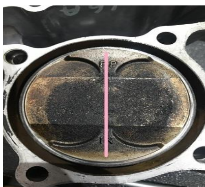
Piston squish measurement area ( where violet line).
