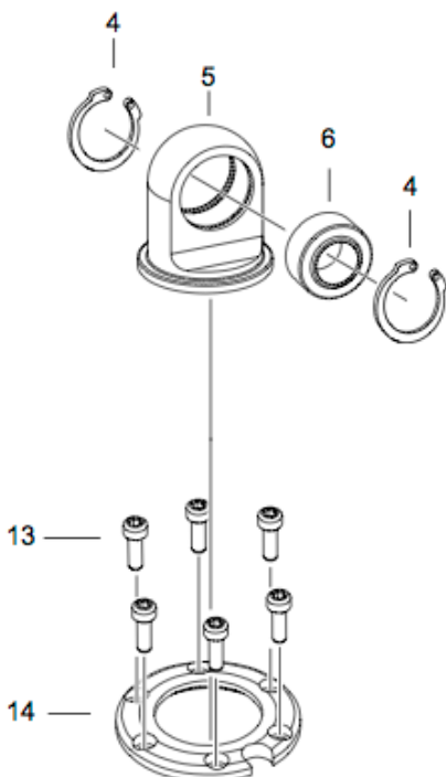
Figure 3 - Top Eye Assembly
