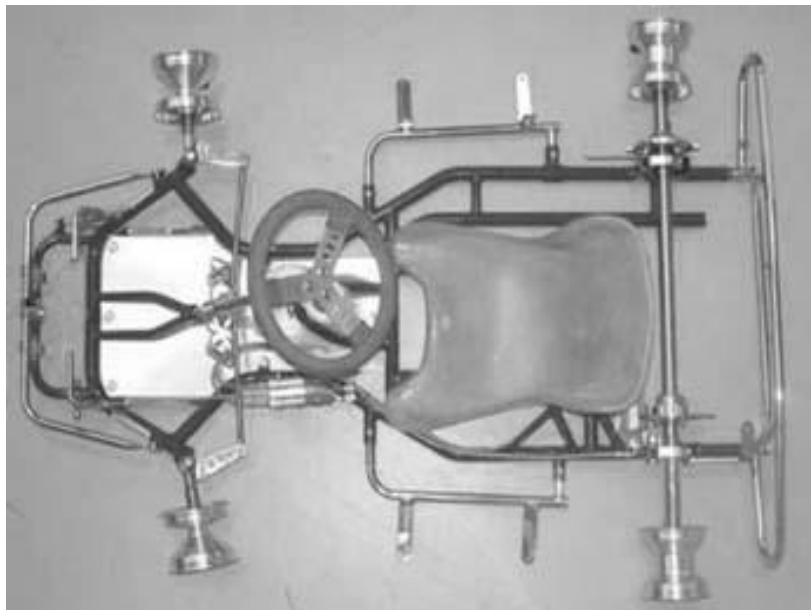
Photo of complete chassis less seat, tyres and bodywork
